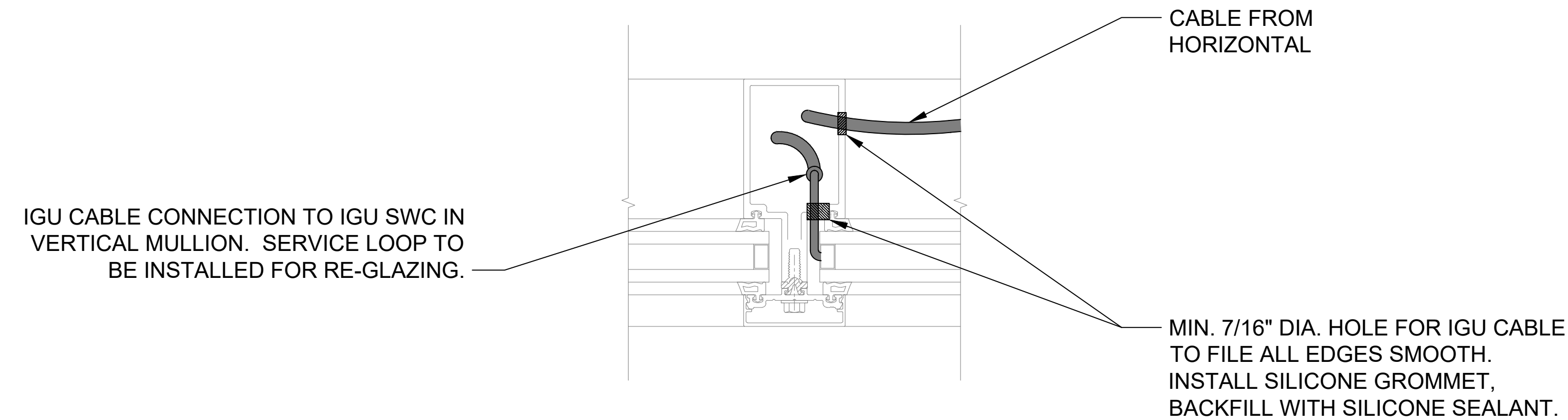
DETAIL 5 VERTICAL MULLION
