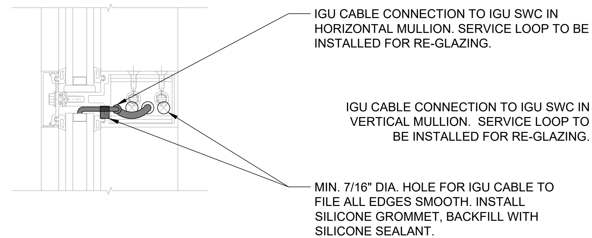
DETAIL 2 HORIZONTAL MULLION
